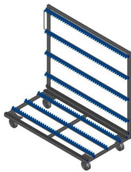
40 slot IGU cart 65" L x 57" H x 35" D 45/64"-1-3/8" slots
